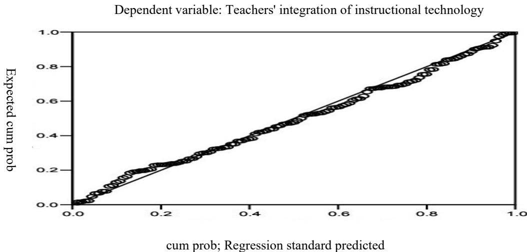
Figure 2. Probability plot
